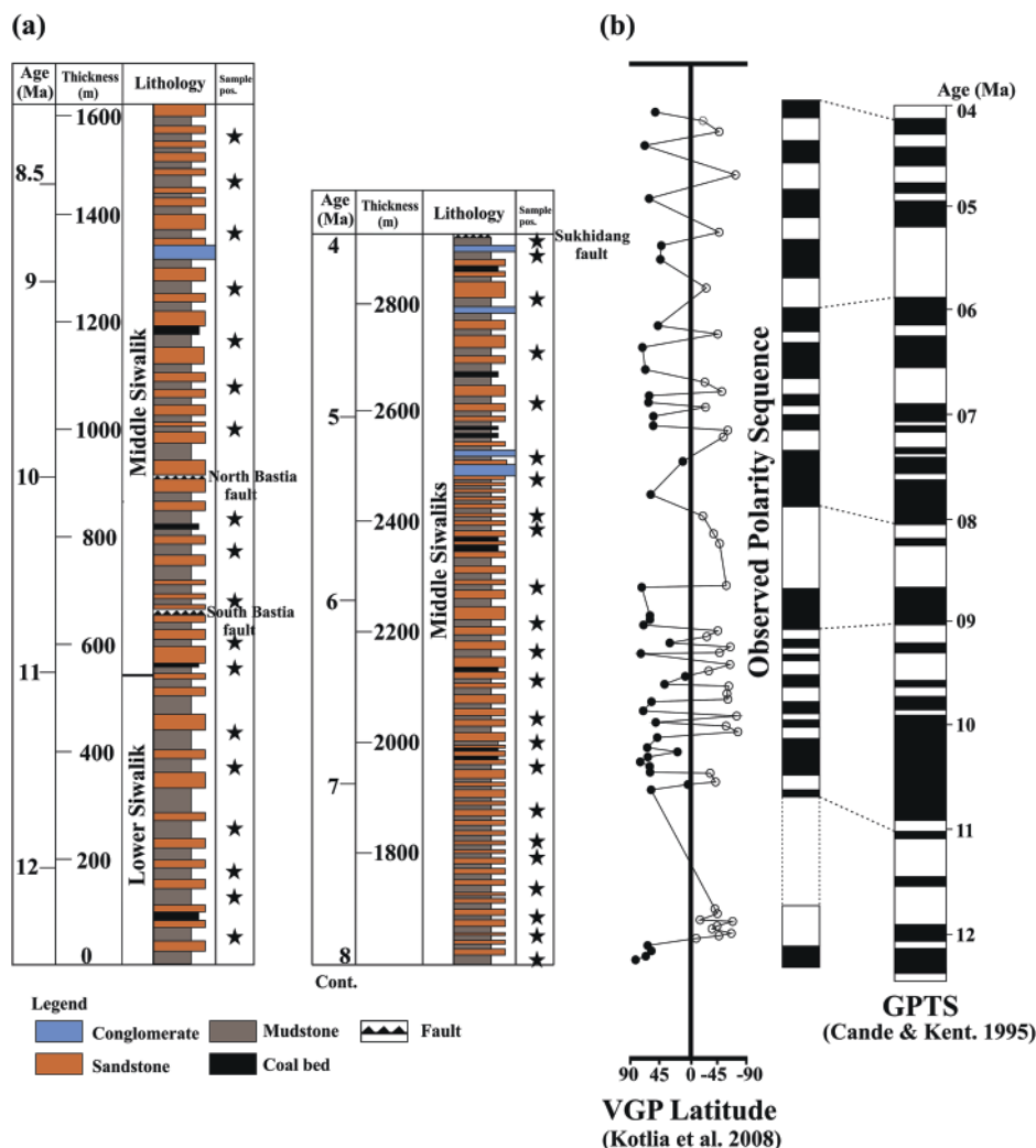
Fig. 5 | Lithostratigraphy and magnetostratigraphy of the TS section of the HFB and correlation to the geomagnetic polarity timescale (GPTS). a Modified Lithology 111 ; b virtual geomagnetic pole (VGP) latitude and paleomagnetic polarity for the TS section 111 and correlation to the GPTS 124 .
